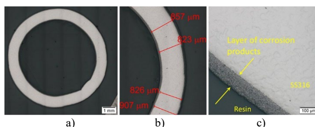
Fig. 9. Macro image of the sample after tests at 950°C (120 h) (a), microstructure with an example of wall thickness measurement (b), and the appearance of the corrosion product layer with a fragment of SS316 (c). Unetched cross-section, light microscopy
