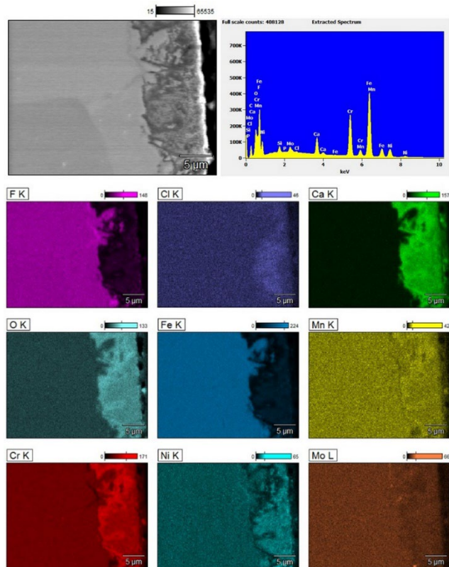
Fig. 7. Microstructure of the sample tested for 120 h at 700°C and elemental distribution maps of components present in the molten salts: F, Cl, Ca, O, as well as primary alloying elements of AISI 316 steel: Fe, Mn, Cr, Ni, Mo
