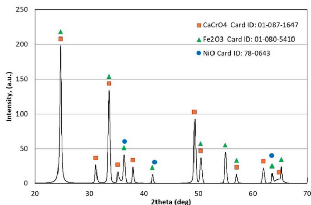
Fig. 13. XRD pattern of the corrosion products formed at 950 °C on the surface of SS316
