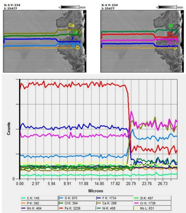
Fig. 8. Results of linear analysis of the microstructure area (sample tested for 120 h at 700°C) on a cross-section containing the corrosion product layer and the base material; SEM
