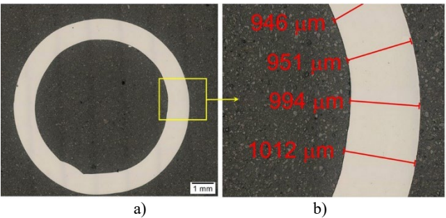
Fig. 3. Macro image of the sample before testing (a) and microstructure with an example of wall thickness measurement (b), unetched cross-section, light microscopy
