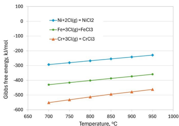
Fig. 15. The Gibbs free energy for the formation reaction of Ni, Fe and Cr chlorides in the temperature range of 700-950°C [22]
