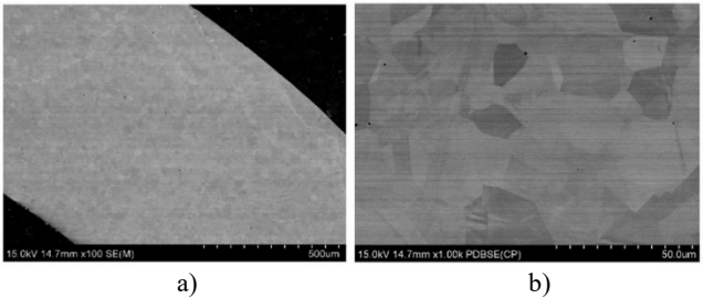
Fig. 4. Microstructure of the sample cross-section before testing: a) magnification 100x, b) magnification 1000x; SEM
