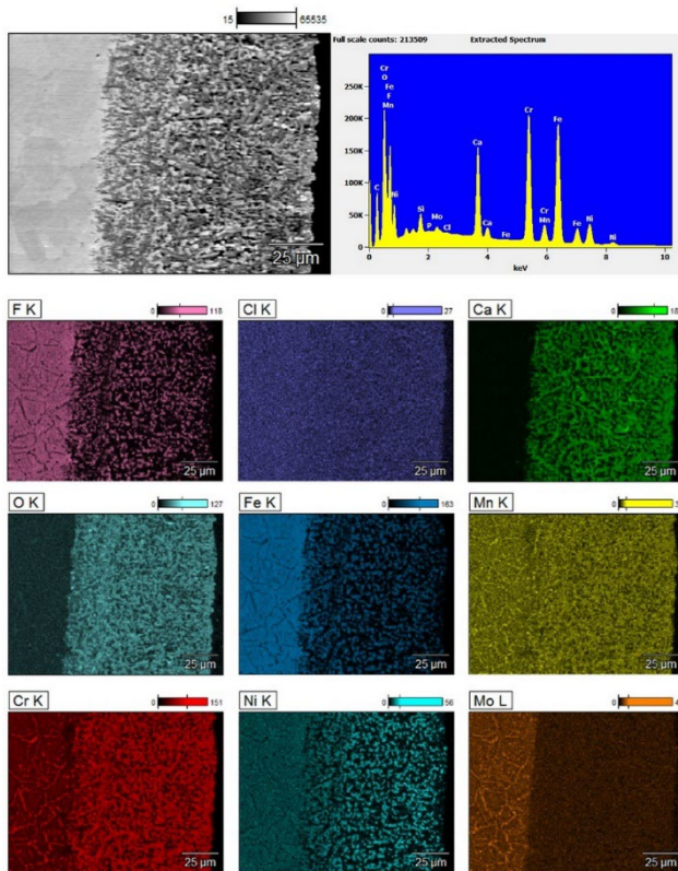
Fig. 11. Microstructure of the sample tested for 120 h at 950°C and elemental distribution maps of components present in the molten salts: F, Cl, Ca, O, as well as primary alloying elements of SS316 steel: Fe, Mn, Cr, Ni, Mo
