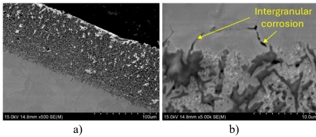
Fig. 10. Microstructure of the sample tested for 120 h at 950°C; image (a) shows the morphology of the corrosion layer, and image (b) displays evidence of intergranular corrosion; SEM
