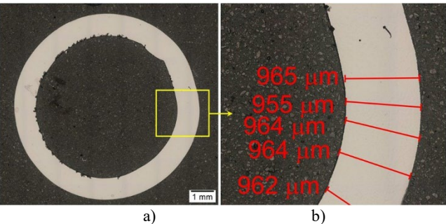
Fig. 5. Macro image of the sample after tests at 700°C (120 h) and microstructure with an example of wall thickness measurement (b), unetched cross-section
