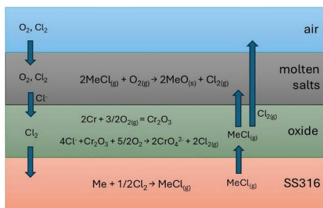
Fig. 14. Schematic diagram of activated oxidation.
