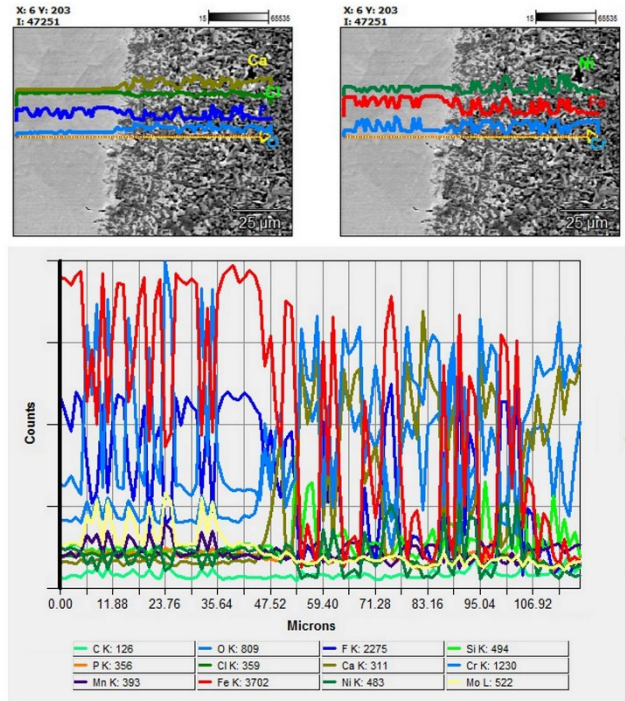
Fig. 12. Results of linear analysis of the microstructure area of the sample tested for 120 h at 950°C, showing a cross-section containing the corrosion layer and the tube material; SEM
