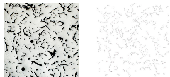
a) microstructure image
