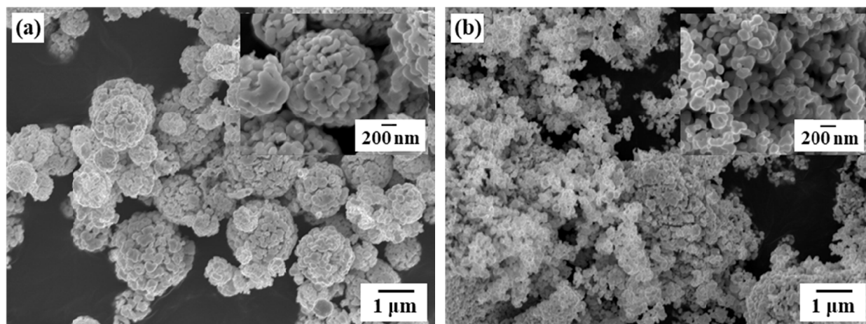
Fig. 3. SEM micrographs of hydrogen-reduced W-Cu composite powders using (a) USP and (b) commercial \text{WO}_3 as raw powders
