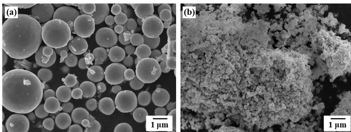
Fig. 1. SEM micrographs of calcined composite powders using (a) USP and (b) commercial \text{WO}_3 as raw powders
