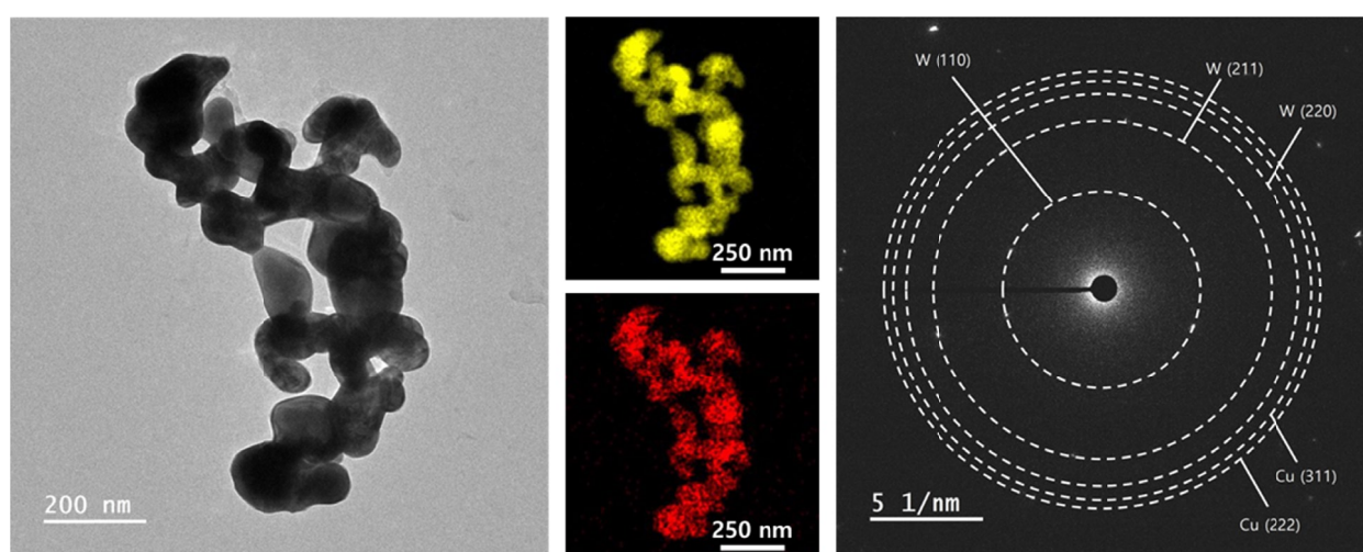
Fig. 4. TEM-EDS-SAED results of hydrogen-reduced W-5 wt.% Cu composite powder
