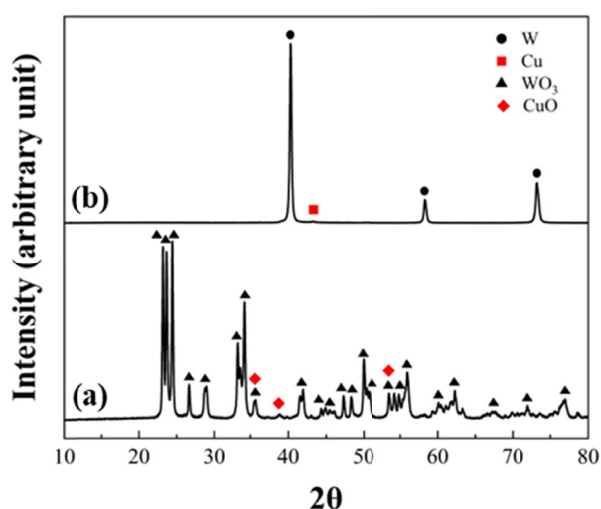
Fig. 2. XRD profiles for the powder mixture of commercial \text{WO}_3 and copper nitrate after (a) calcination at 300°C in air and (b) reduction at 800°C in hydrogen atmosphere
