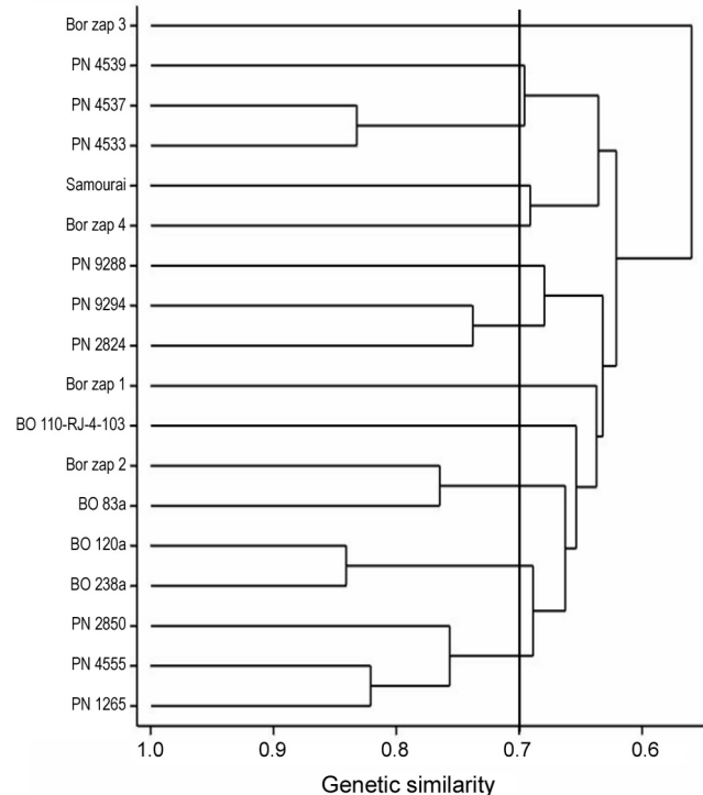
Fig. 6. Dendrogram for 18 parental lines of winter oilseed rape ( B. napus ) constructed for all markers.
