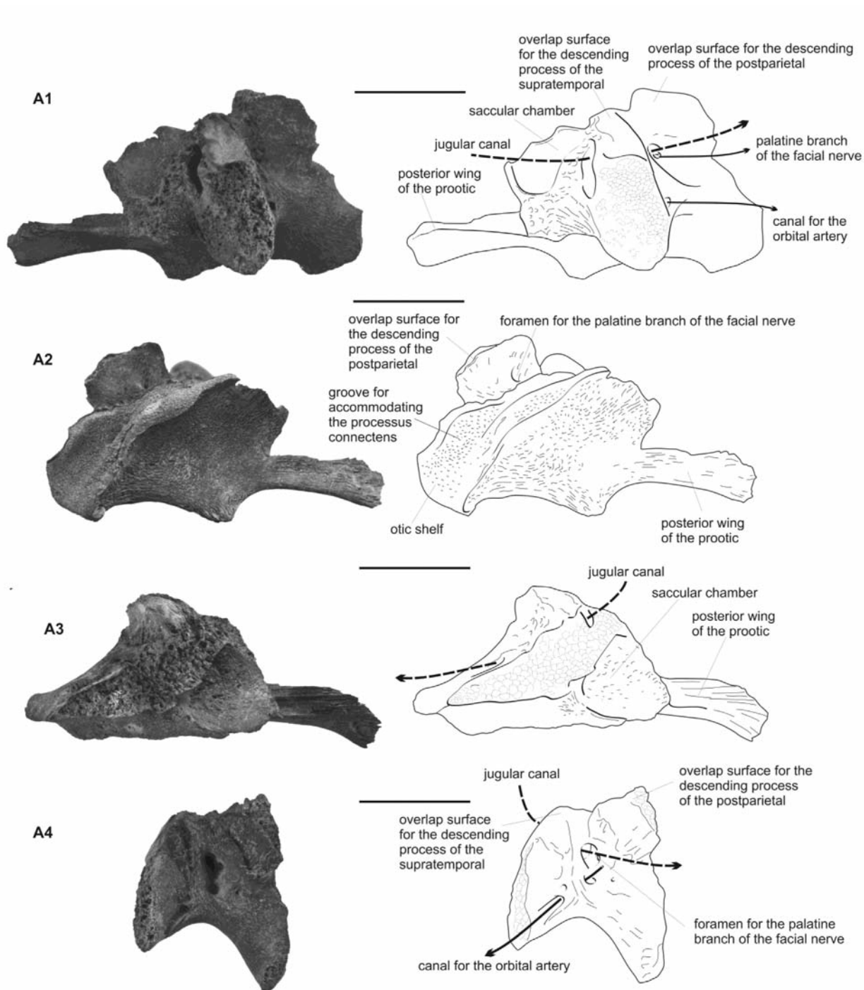
Text-fig. 5. Photographs and semi-interpretative line drawings of the right prootic of the actinistian fish Dobrogeria aegyssensis gen. et sp. nov., NHMW 2013/0609/0005 (holotype) in lateral (A1), medial (A2), dorsal (A3) and anterior (A4) views; Tulcea Veche Limestone, Lower Spathian, Tulcea. Scale bars: 20 mm
