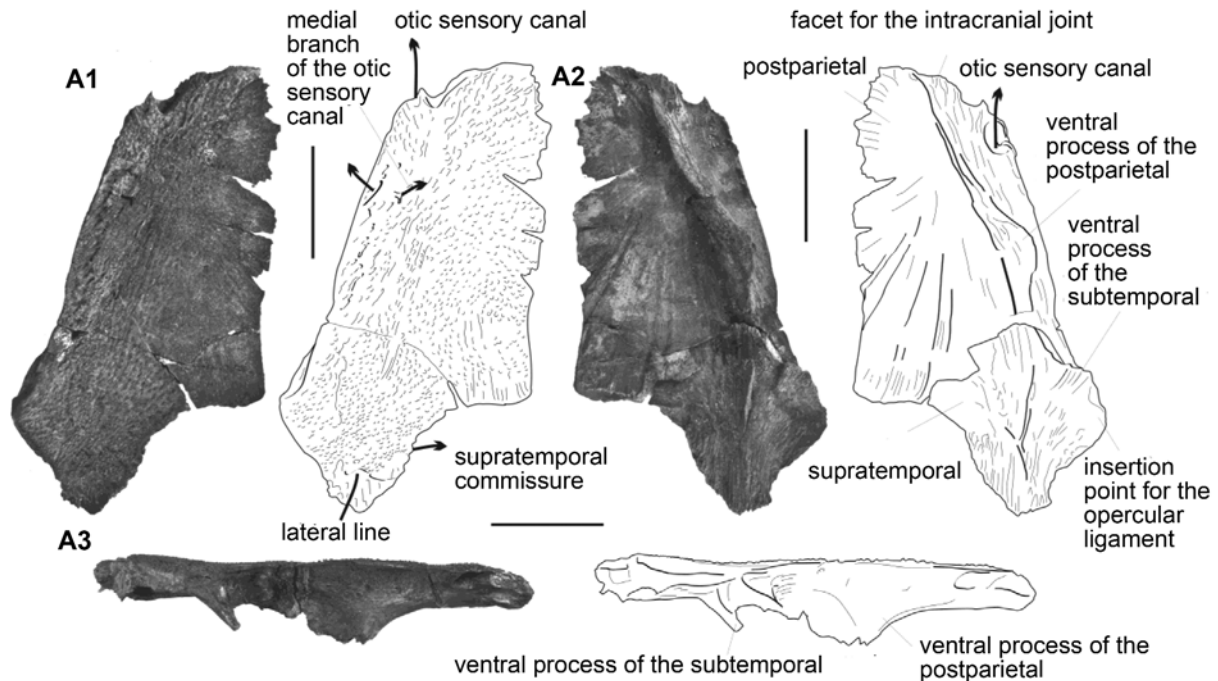
Text-fig. 3. Photographs and semi-interpretative line drawings of left half of the skull roof of the postparietal shield of the actinistian fish Dobrogeria aegyssensis gen. et sp. nov., NHMW 2013/0609/0002 (holotype) in dorsal (A1), ventral (A2) and lateral (A3) views; Tulcea Veche Limestone, Lower Spathian, Tulcea. Scale bars: 20 mm
