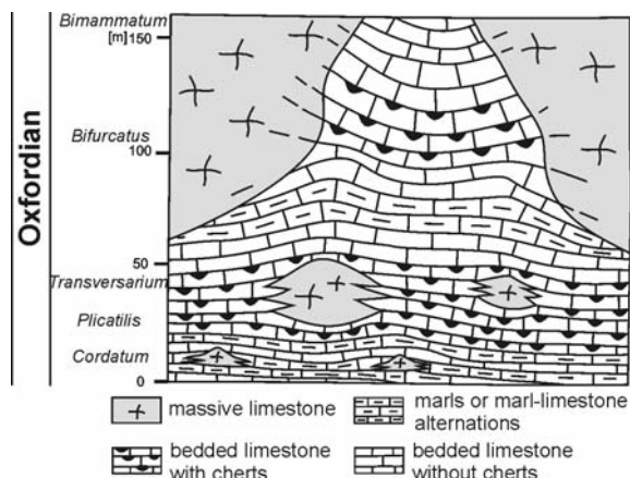
Text-fig. 3. Stratigraphic column of Oxfordian strata in the Sokole Hills (on the basis of Heliasz et al. 1982, 1987). Positions of ammonite zones are approximate
