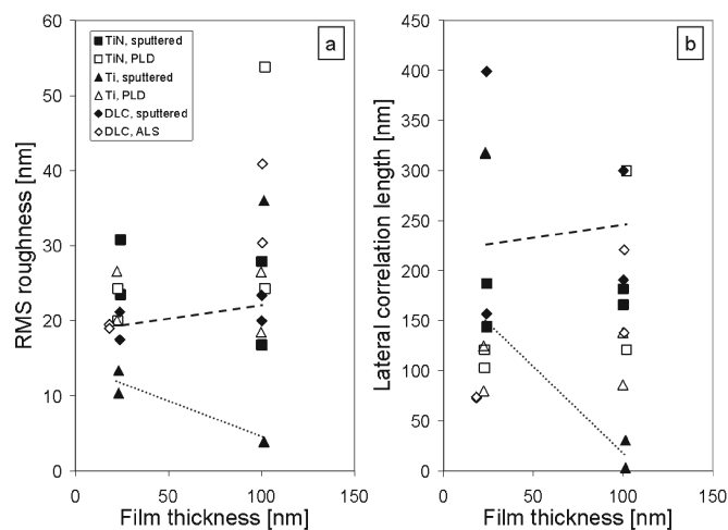
Fig. 11. a) RMS roughness and b) lateral correlation length (LCL) of different thin film materials, deposited by different deposition techniques (at different vapour energy), in dependency of their thickness on smooth PU substrates. Two values of RMS and LCL were measured independently and are given in the diagrams
