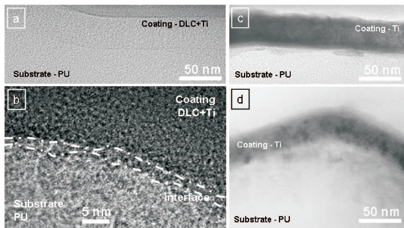
Fig. 4. TEM images of nucleation and growth structures close to the interface of 50 nm thick PVD coatings on polyurethane (PU): a), b) Magnetron sputtered titanium-doped diamond-like carbon (DLC, a-C:H:Ti) (b: magnified detail of a)), c) magnetron sputtered Ti, and d) PLD Ti
