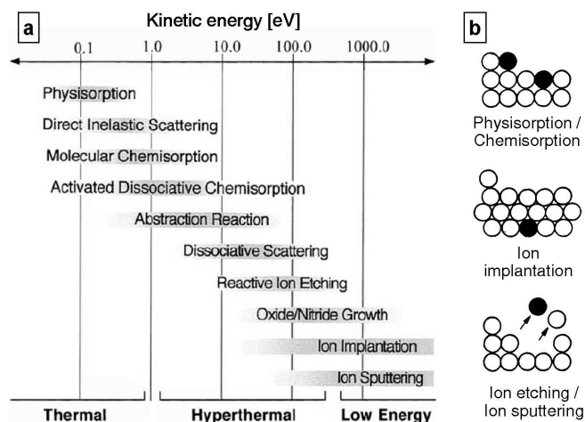
Fig. 1. a) Fundamental processes occurring in the interaction between vaporized (ionised) atoms/molecules and the solid surfaces. The shaded region designates the ion kinetic energy range over which the associated process is evident; b) The schematics present simplified the most important processes of this interaction (adapted from Refs. 1, 7, 9)
