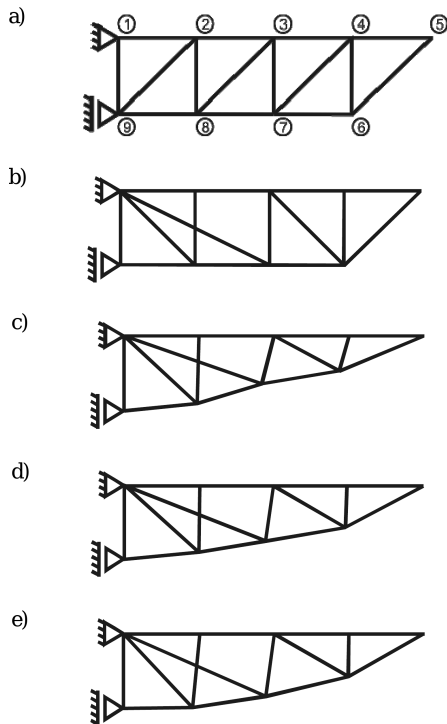
Fig. 3. Optimization of the truss: a) The initial design, b) The optimal topology, c) The optimal design for the first loading case, d) The optimal design for the second loading case, e) The optimal design for both loading cases
