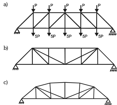
Fig. 2. Optimization of the truss: a) The initial design, b) The optimal topology, c) The optimal design
