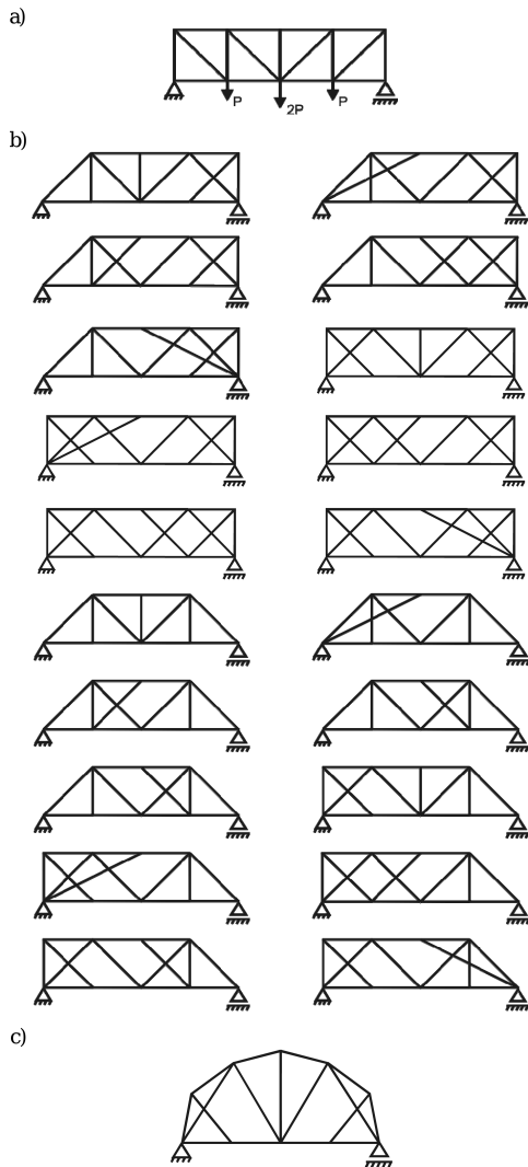
Fig. 1. Optimization of the truss: a) the initial design, b) selected optimal topologies, c) the optimal design
