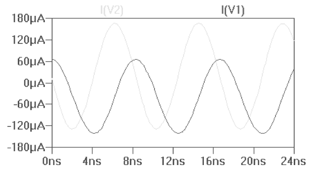
Fig. 24. Output currents of the quadrature oscillator
