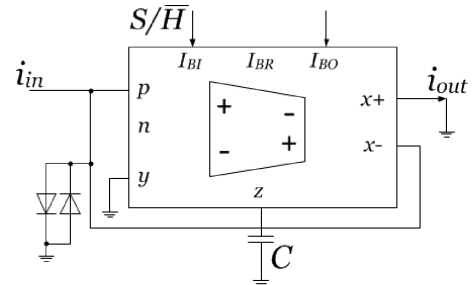
Fig. 22. MCDTA based track and hold circuit
