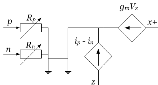
Fig. 1. CDTA equivalent circuit
