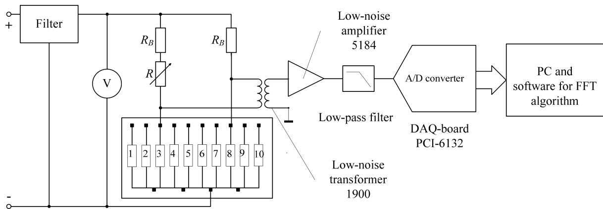
Fig. 1. The measurement setup for noise studies in the Ni-P thin-film resistors embedded in PCBs
