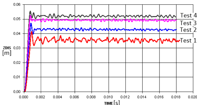
Fig. 14. Plots for central node displacement for individual tests
