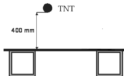
Fig. 8. The scheme of the test plate
