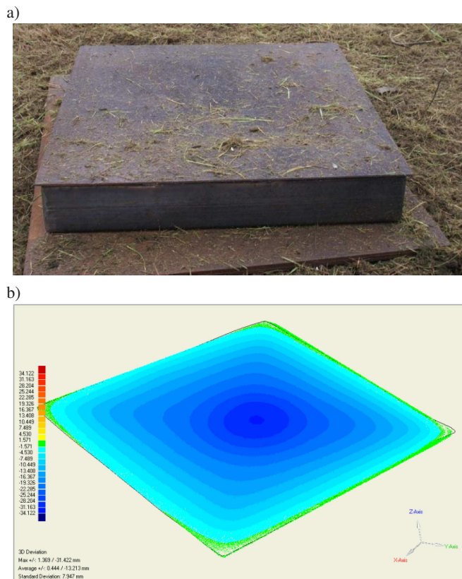
Fig. 10. Experimental zone after the experiment – Test 1: a) system after explosion, b) deformation map obtained by measuring with a 3D scanner
