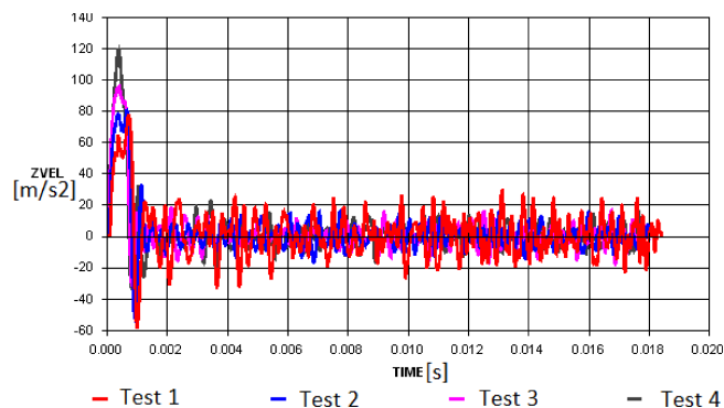
Fig. 17. Speed of the node located on the upper wall of the object (the plane of symmetry)
