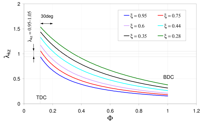
Fig. 8. Excess air-fuel ratio of mixture in prechamber during compression process for different values of degree of filling of prechamber at BDC, (prechamber powered by rich mixture of \lambda_{k_{co}} = 0.15 for \lambda_c = 2.0 )
