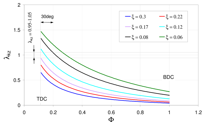
Fig. 9. Excess air-fuel ratio of mixture in prechamber during compression process for different values of degree of filling of prechamber at BDC, (prechamber powered by pure fuel of \lambda_{k_{co}} = 0 for \lambda_c = 2.0 )
