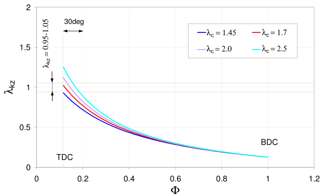
Fig. 7. Excess air-fuel ratio of mixture in prechamber during compression process for different values of excess air-fuel ratio in cylinder, (prechamber powered by pure fuel of \lambda_{k_{co}} = 0 for \xi = 0.12 )
