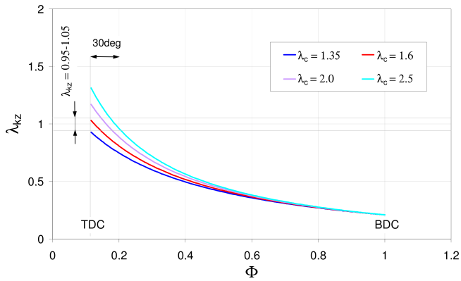
Fig. 6. Excess air-fuel ratio of mixture in prechamber during compression process for different values of excess air-fuel ratio in cylinder, (prechamber powered by rich mixture of \lambda_{k_{co}} = 0.15 for \xi = 0.6 )
