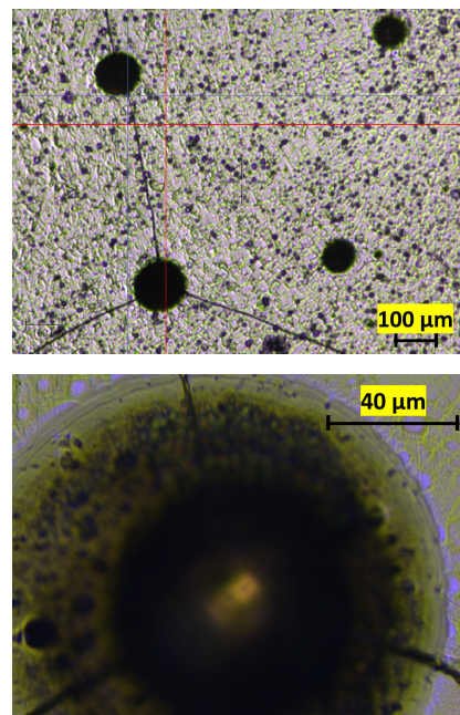
Fig. 9. Ni-W coating after 1700 N
