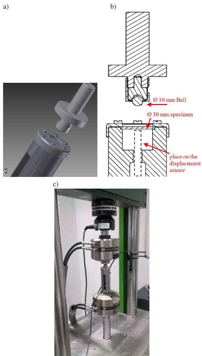
Fig. 3. Handle designed and used in experiments
