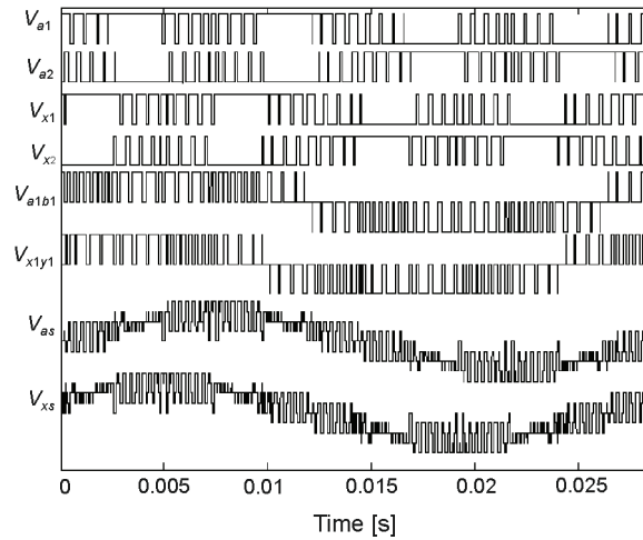
Fig. 6. Pole voltages V_{a1} , V_{a2} and V_{x1} , V_{x2} , line-to-line voltages V_{a1b1} and V_{x1y1} , and phase voltages V_{as} and V_{xs} of dual three-phase system with discontinuous synchronized PWM ( F = 35 Hz, V_{dc1} = V_{dc2} = V_{dc3} = V_{dc4} , m_1 = m_2 = m_3 = m_4 = 0.7 , F_s = 1 kHz)
