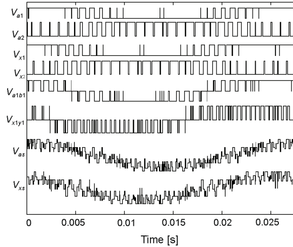
Fig. 8. Pole voltages V_{a1} , V_{a2} and V_{x1} , V_{x2} , line-to-line voltages V_{a1b1} and V_{x1y1} , and phase voltages V_{as} and V_{xs} of dual three-phase system with continuous synchronized PWM ( F = 35 Hz, V_{dc1} = 0.7 V_{dc2} , V_{dc3} = 0.7 V_{dc4} , V_{dc2} = V_{dc4} , m_1 = m_3 = 0.933 , m_2 = m_4 = 0.7 , F_s = 1 kHz)
