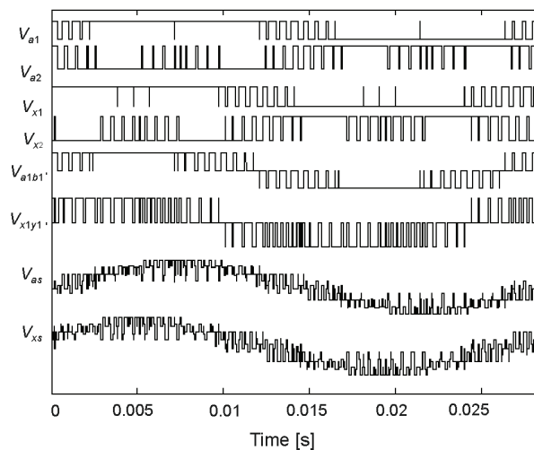
Fig. 12. Pole voltages V_{a1} , V_{a2} and V_{x1} , V_{x2} , line-to-line voltages V_{a1b1} and V_{x1y1} , and phase voltages V_{as} and V_{xs} of dual three-phase system with discontinuous synchronized PWM ( F = 35 Hz, V_{dc1} = 0.8V_{dc2} , V_{dc2} = 0.9V_{dc4} , V_{dc3} = 0.75V_{dc4} , m_1 = 0.97 , m_2 = 0.777 , m_3 = 0.933 , m_4 = 0.7 , F_s = 1 kHz)
