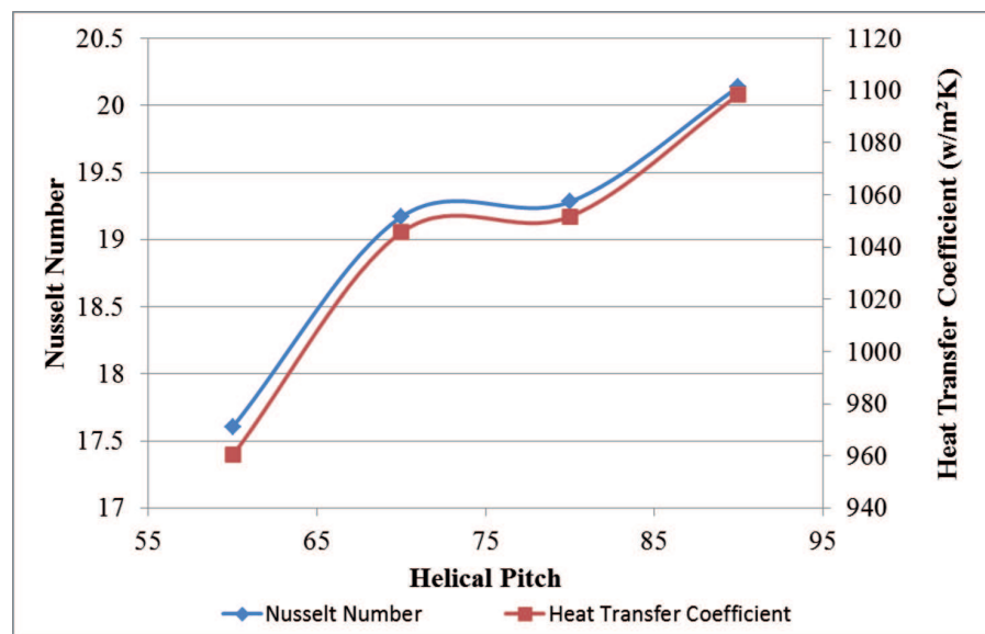
Fig. 12. The effect of pitch variation on Nusselt Number and heat transfer coefficient (a = 12.5)
