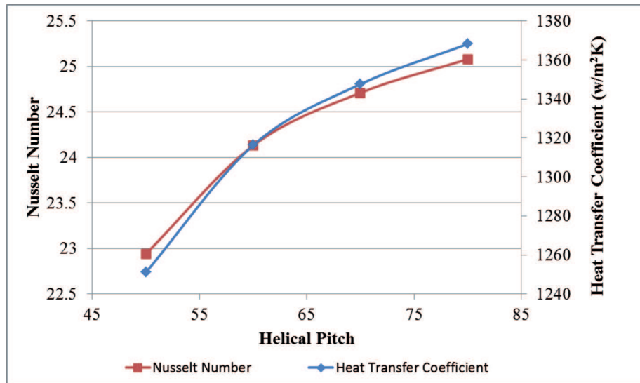
Fig. 11. The effect of pitch variation on Nusselt Number and heat transfer coefficient (a = 10)
