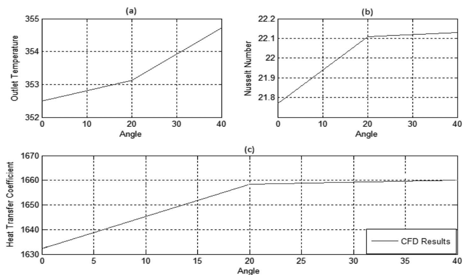
Fig. 3. The effect of the taper angle on the temperature, heat transfer coefficient and Nusselt number ( R = 70 )
