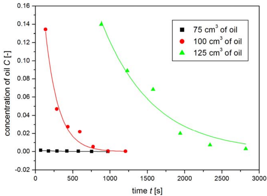
Fig. 7. The dependence of oil concentration in the samples as the function of time, sand, fraction 250 ÷ 400 μm
