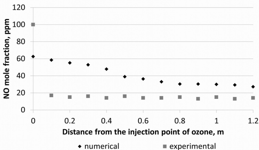
Fig. 8. Axial profiles of the numerically and experimentally determined NO mole fractions for counter-current ozone injection and X = 1.5
