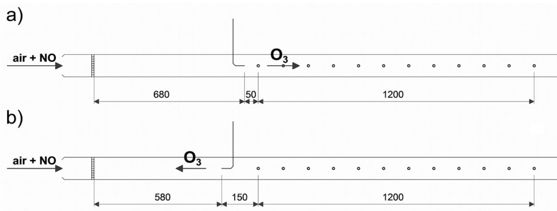
Fig. 1. Measurement locations in the reactor a) co-current injection, b) counter-current injection
