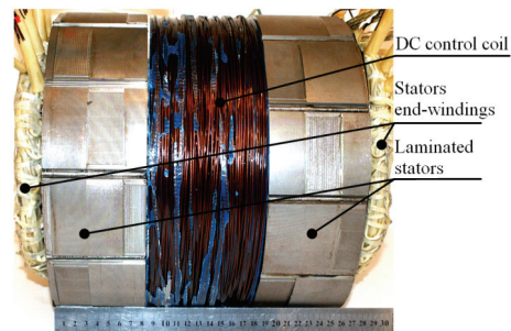
Fig. 10. Stator of ECPMS-machine
