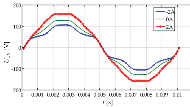
Fig. 13. Back-EMF phase-to-phase waveforms at 1000 rpm for the selected values of the DC control coil current
