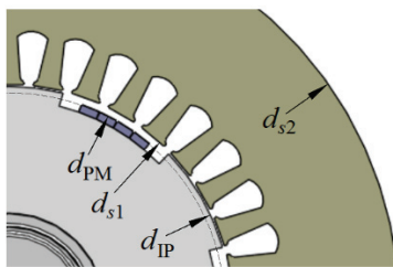
Fig. 5. Cross section of the ECPMS-machine
