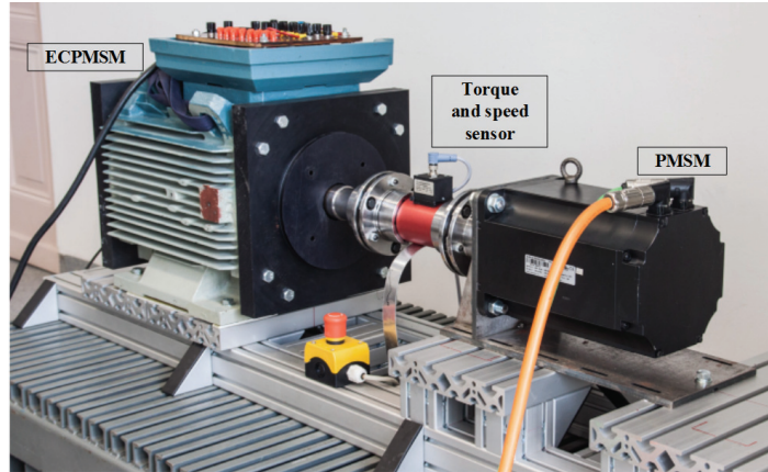
Fig. 12. Experimental set-up
