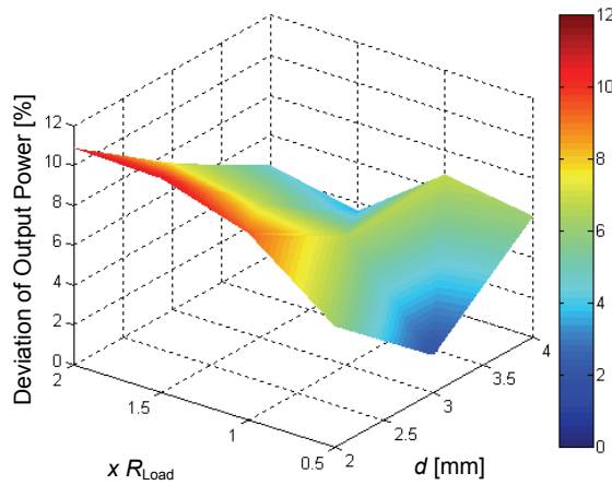
Fig. 9a. Deviation between measured and simulated output power P_{out}
