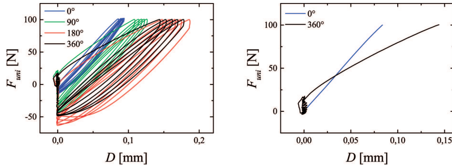
Fig. 11. Left: Influence of pretorsion on the behavior in cyclic tensile test. Right: Loading paths of the first cycles for 0° and 360° pretorsion
