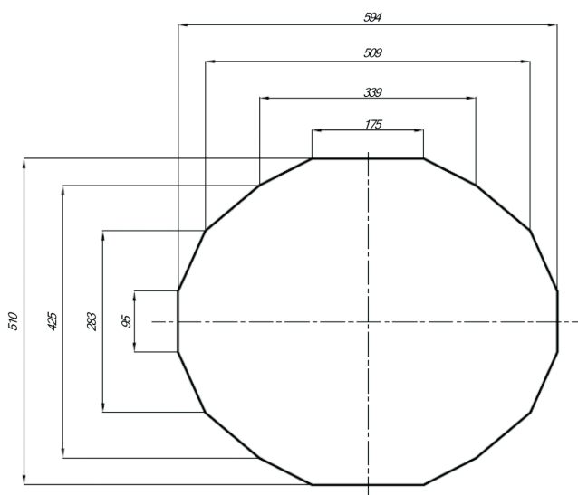
Fig. 2. Geometry of a blank used for deep drawing
