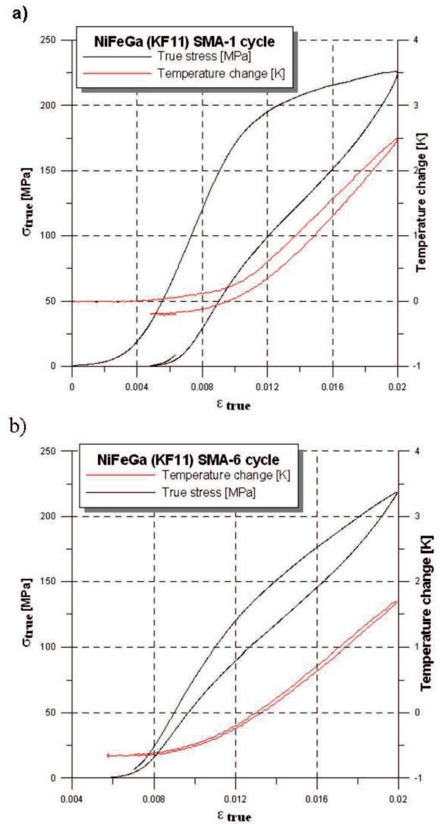
Fig. 6. Stress-strain and temperature-strain curves obtained for 1 st and 6 th direct cycles of compression polycrystalline NiFeGa with strain rate 10^{-2} s^{-1} and within the strain range 2%
