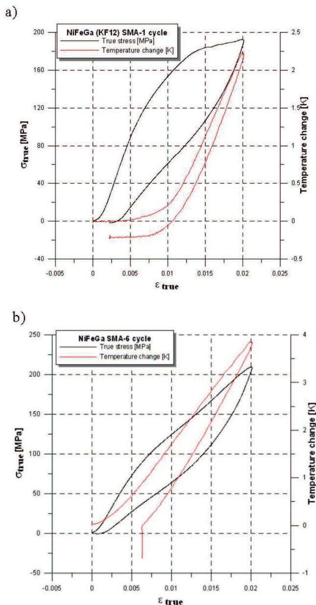
Fig. 4. Stress-strain and temperature-strain curves obtained for 1 st and 6 th cycles of compression polycrystalline NiFeGa with strain rate 10^{-2}\text{s}^{-1} and within the strain range 2%
