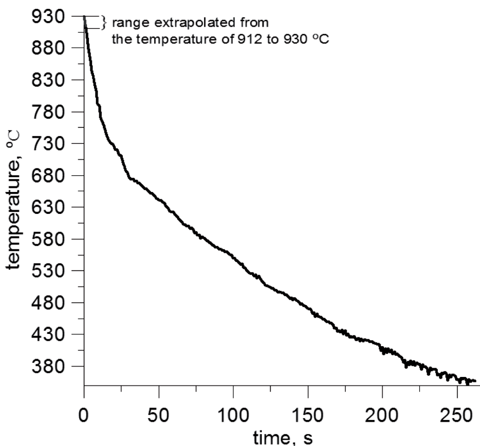
Fig. 1. Measured cooling curve of the steel rod niobium microalloyed temperature 930 to 350°C
