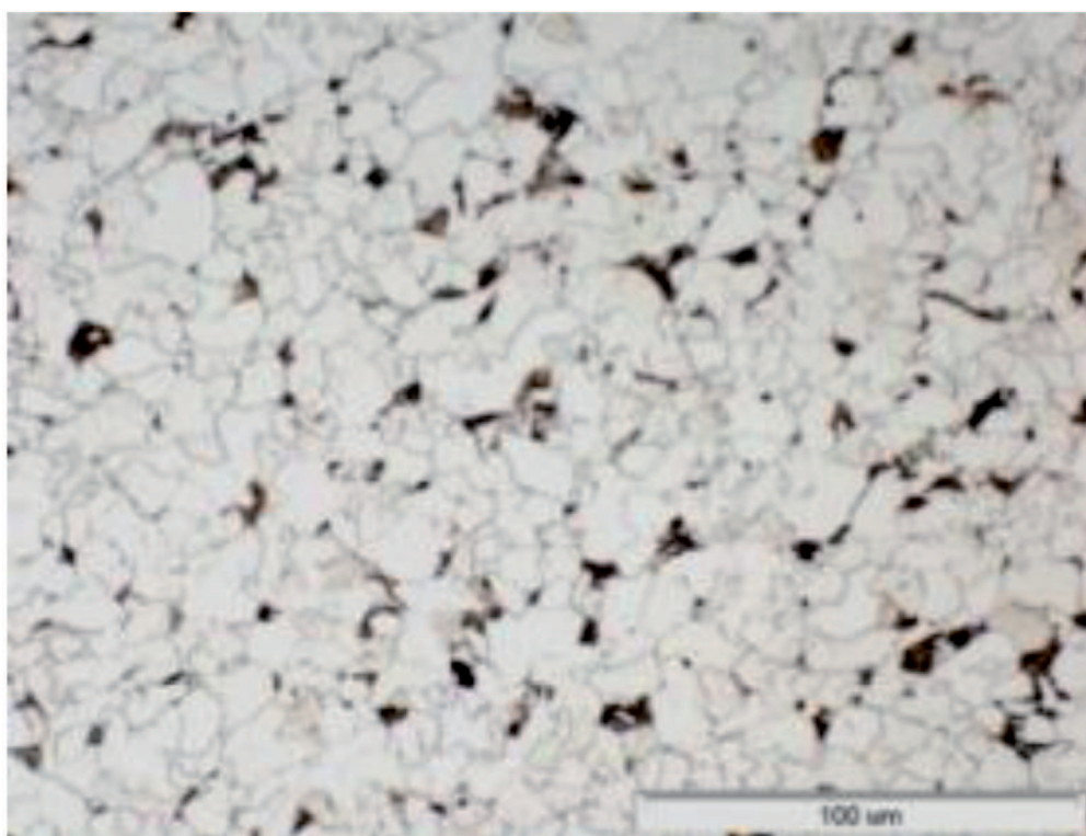
Fig. 4. Microstructure of the rolled steel rod microalloyed niobium after cooling to a temperature of 350° C
