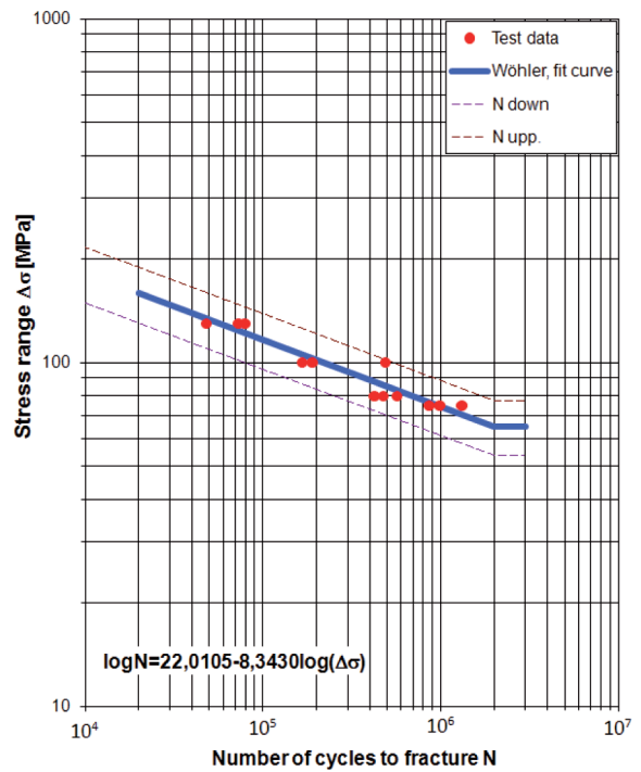
Fig. 11. Wöhler's line for 8 mm-thick joints welded with T3 tool with machined post-weld surface
