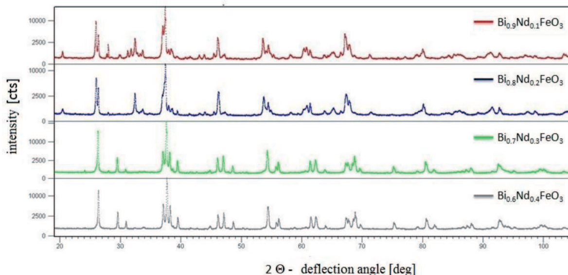
Fig. 3. Comparison of X-ray diffraction patterns for \text{Bi}_{1-x}\text{Nd}_x\text{FeO}_3 ceramics (Co-radiation)
