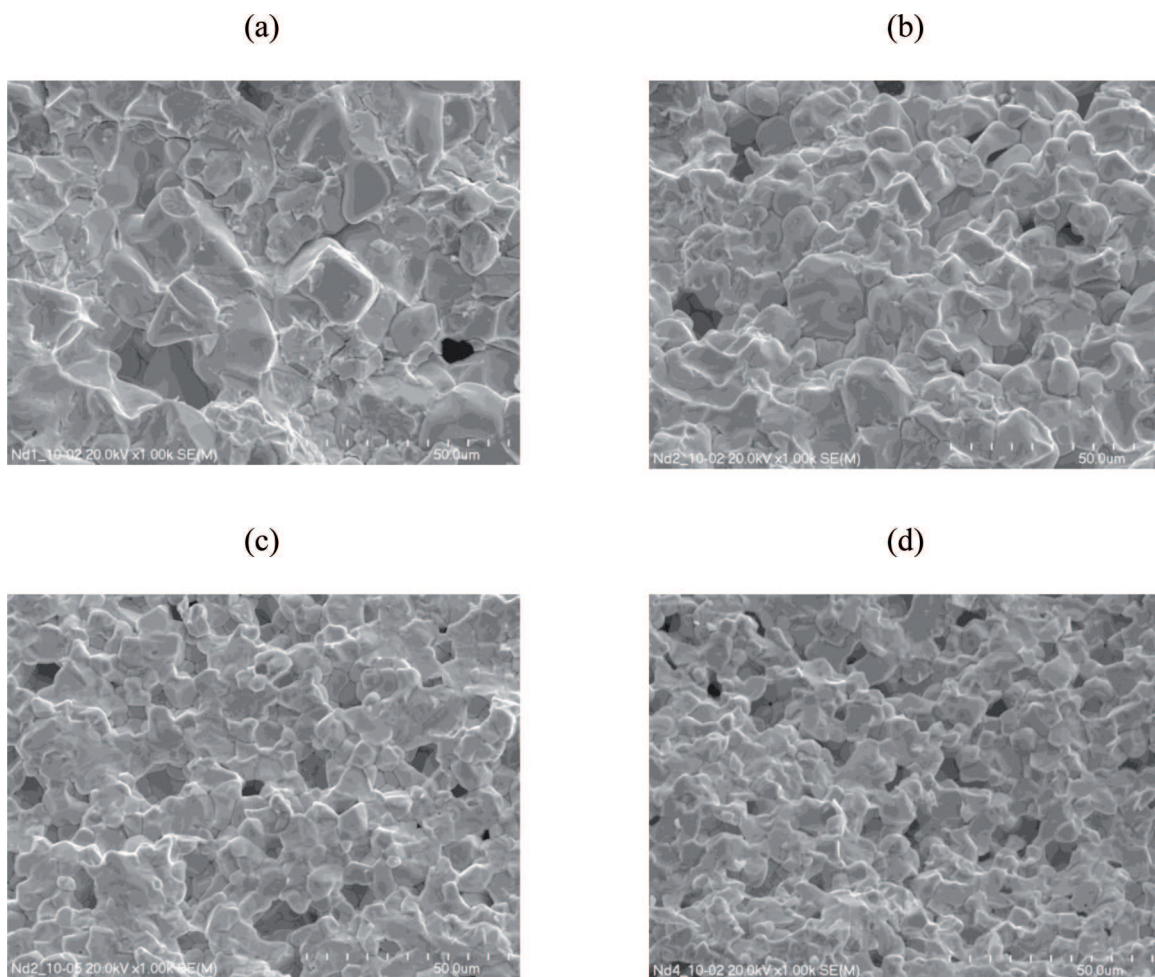
Fig. 2. SEM micrographs of \text{Bi}_{1-x}\text{Nd}_x\text{FeO}_3 sintered at T=1000^\circ\text{C} for t=24\text{h} , \text{Bi}_{0.9}\text{Nd}_{0.1}\text{FeO}_3 (a), \text{Bi}_{0.8}\text{Nd}_{0.2}\text{FeO}_3 (b), \text{Bi}_{0.7}\text{Nd}_{0.3}\text{FeO}_3 (c), \text{Bi}_{0.6}\text{Nd}_{0.4}\text{FeO}_3 (d)
