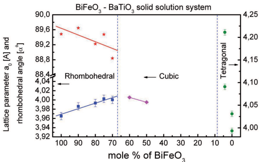
Fig. 2. Phase diagram of \text{BiFeO}_3 - \text{BaTiO}_3 - prepared on the base of data from [12,13]
