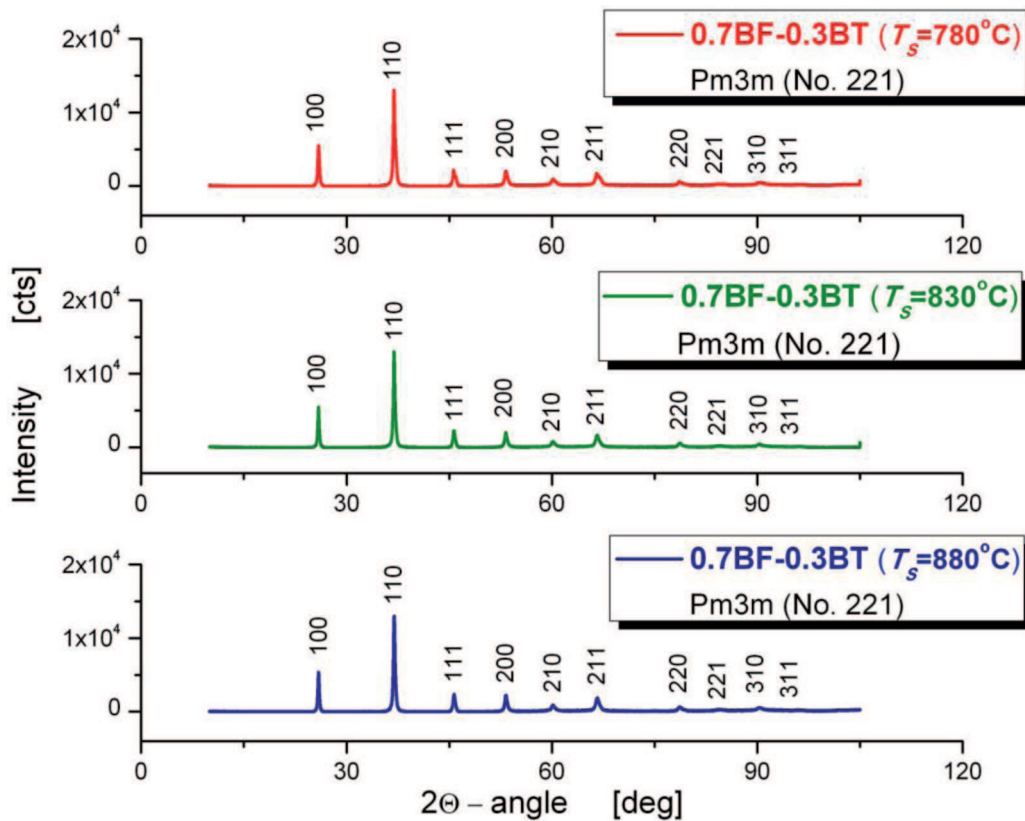
Fig. 7. Comparison of X-ray diffraction patterns for 0.7BF–0.3BT ceramics fabricated of different technological conditions ( T_s - sintering temperature)
