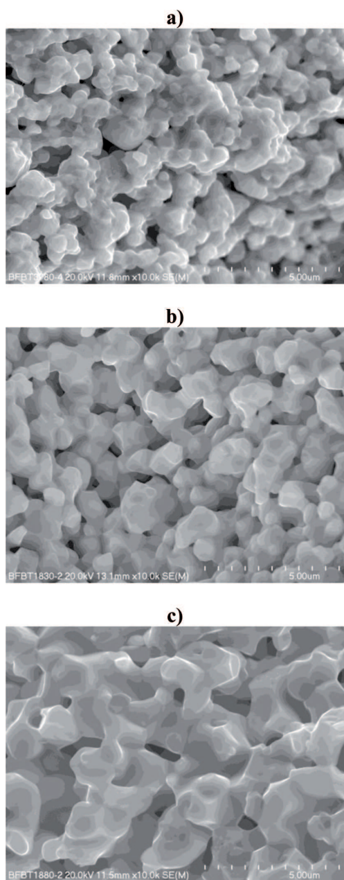
Fig. 6. SEM photographs of the microstructure fracture of 0.7\text{BiFeO}_3\text{-}0.3\text{BaTiO}_3 ceramics specimens: (a) sintered at T=780^\circ\text{C} , (b) sintered at T=830^\circ\text{C} , (c) sintered at T=880^\circ\text{C} ( \times 10\,000 )
