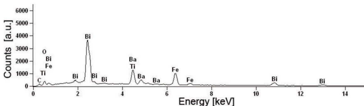
Fig. 5. EDS spectrum of 0.7\text{BiFeO}_3\text{-}0.3\text{BaTiO}_3 ceramics
