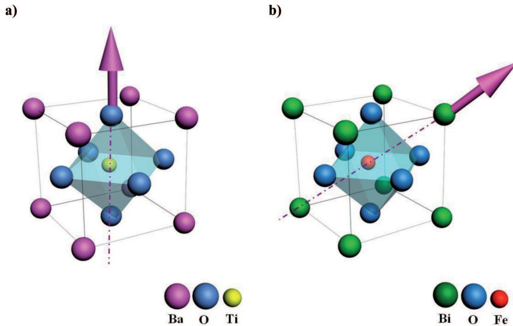
Fig. 1. Perovskite-type structure \text{ABO}_3 of \text{BaTiO}_3 adopting tetragonal symmetry (a) and \text{BiFeO}_3 exhibiting rhombohedral symmetry (b). Direction of the polarization vector P is also shown
