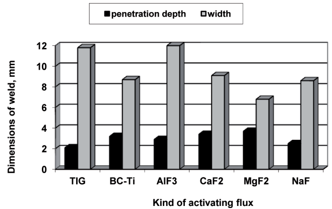
Fig. 3. Impact of type and content of activating flux on penetration depth and width of welds produced with TIG and A-TIG methods on Grade 2 titanium sheet
