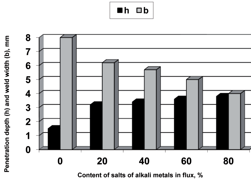
Fig. 1. Relation between dimensions of welds produced with TIG method during welding of Grade BT 15 titanium-based alloy and content of salts of alkali metals in flux ( I = 100 \text{ A} ; U = 9 \text{ V} ; V_w = 15 \text{ m/h} ) [2]
