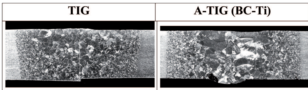
Fig. 5. Macrostructure of butt joints of 5 mm-thick Grade 2 titanium produced by means of TIG and A-TIG methods (Kroll's reagent)
