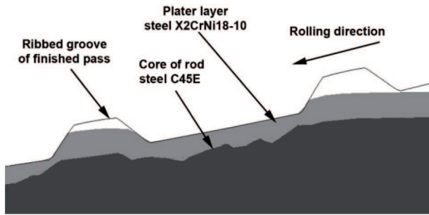
Fig. 11. Forming of the bimetallic round bar ribs in the finishing ribbed groove
