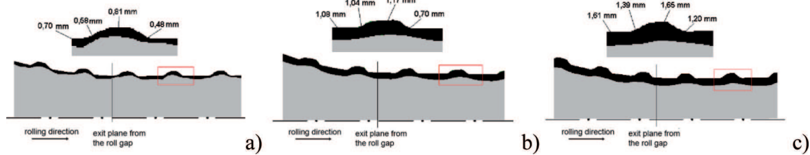
Fig. 10. Distribution of layer surface thickness on the longitudinal cross in deformation zone during bimetallic bar rolling using flat oval pass with the platter layer containing: a) 17.3 %; b) 25.5 %; c) 33.1 %
