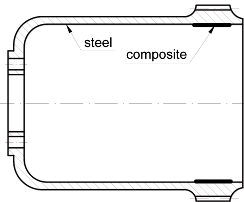
Fig. 2. Construction of a steel-composite cup-type flexspline
