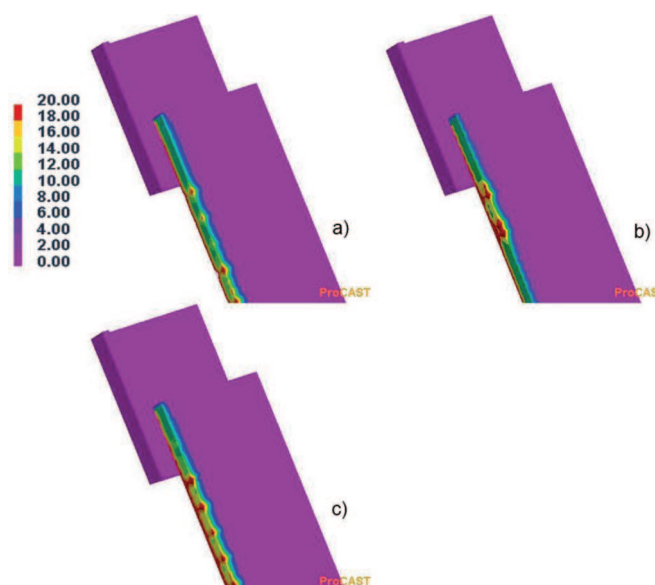
Fig. 6. The effective stress distribution (MPa) for: a) the reference parameters, b) increased casting speed, c) increased the intensity of cooling
