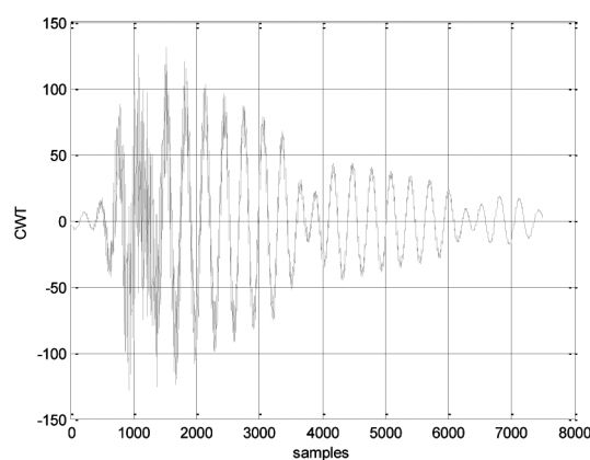
Fig. 15. Wavelet distribution time section for acceleration of the vibrations recorded by sensor A on the steel ball impact in point 1
