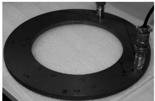
Fig. 7. Subject of studies and arrangement of measurement points
