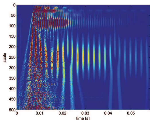
Fig. 11. Distributions of wavelet coefficients obtained for measurement point B on excitation in point 6 (steel disk)
