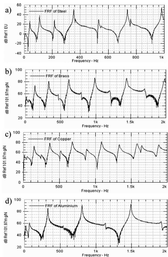
Fig. 1. Frequency response function of: a) steel, b) brase, c) copper, d) aluminum [17]
