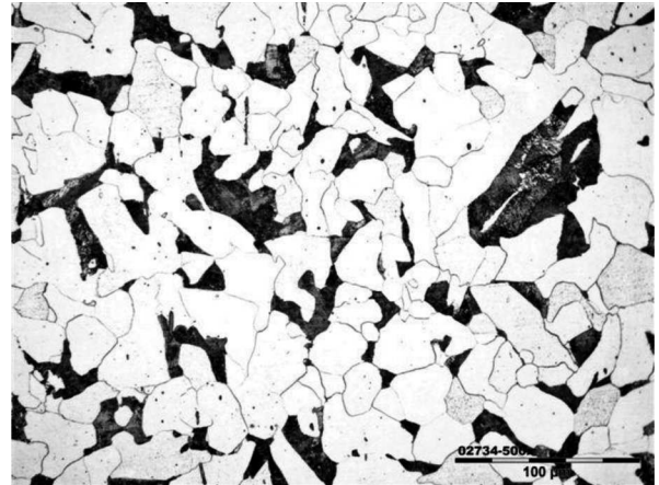
Fig. 6. ST3S steel - fine-grained ferritic-pearlitic structure (magnification of 500x)
