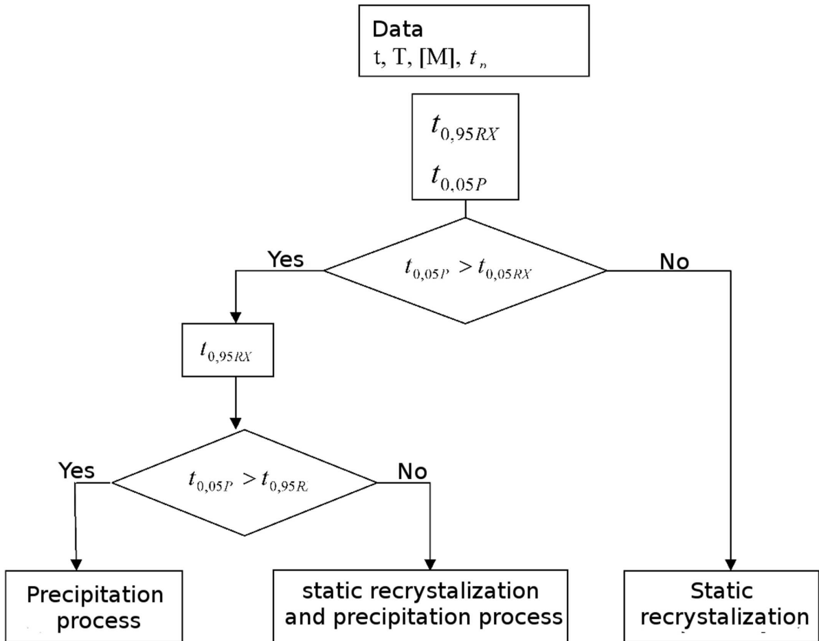
Fig. 3. Algorithm of choosing the main thermomechanical process taking place in the material
