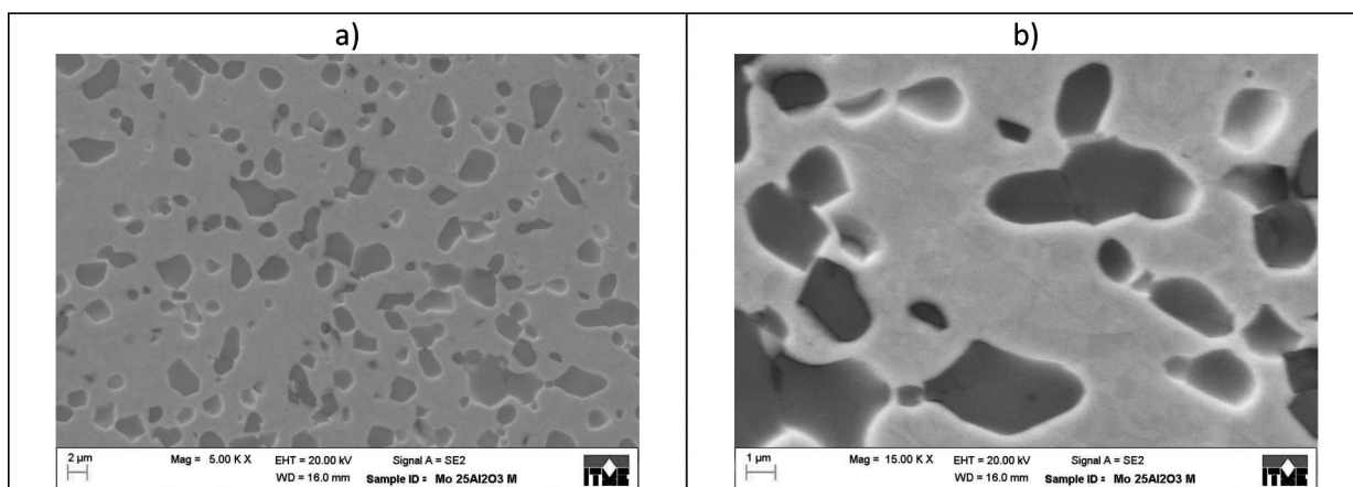
Fig. 4. SEM images of hot pressed Mo-25Al 2 O 3 composites (T=1600°C, p=30 MPa, t=30 min)
