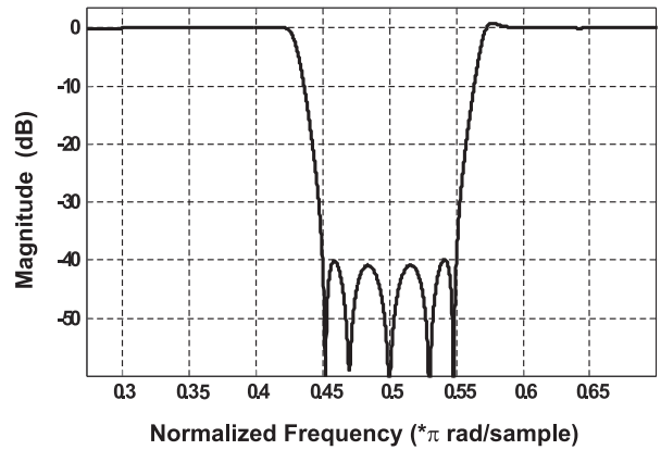
Fig. 7. Magnitude frequency response of the bandstop filter.
