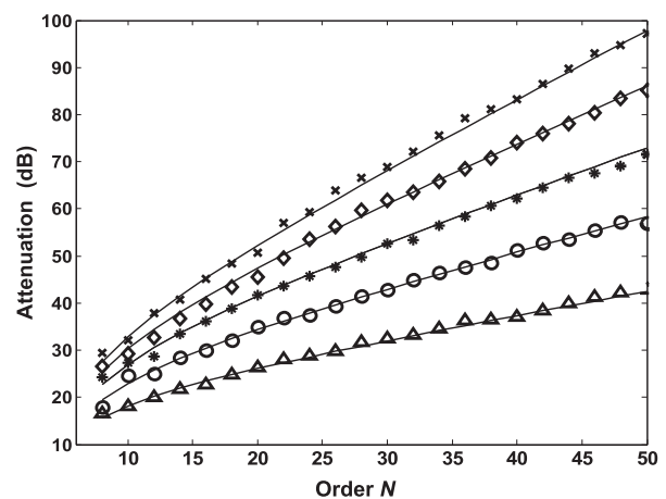
Fig. 2. Approximation of the average values of the stopband attenuation versus N for the lowpass filters with M = 2 and with \omega_t as parameter: \omega_t = 0.04\pi ( \Delta ), \omega_t = 0.07\pi ( \circ ), \omega_t = 0.1\pi ( * ), \omega_t = 0.13\pi ( \diamond ), \omega_t = 0.16\pi ( \times ).
