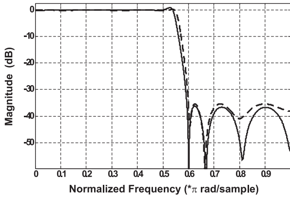
Fig. 5. Magnitude frequency response of lowpass filters designed by algorithm from [11] (solid line) and from [8] (dashed line).
