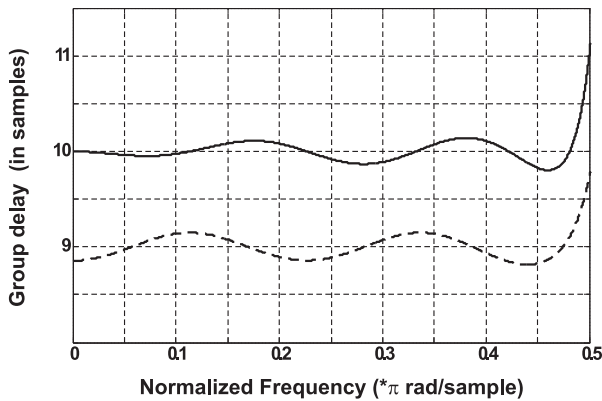
Fig. 6. Group delay response in passband for lowpass filters designed by algorithm from [11] (solid line) and from [8] (dashed line).
