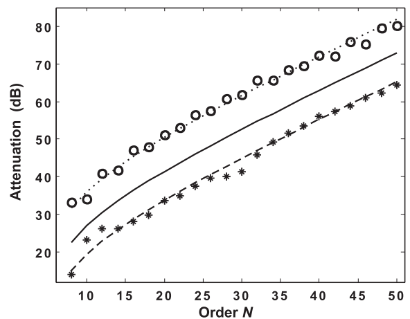
Fig. 8. Relationship A_s = f_2(N) for lowpass filters with M = 2 , \omega_t = 0.1\pi , \omega_p = 0.4\pi and W_p = 1 , W_s = 10 (o), W_p = 5 , W_s = 1 (*). Solid line denotes approximation by (6) for W_p = W_s = 1 , dotted line=solid line+9 dB, dashed line=solid line-6 dB.
