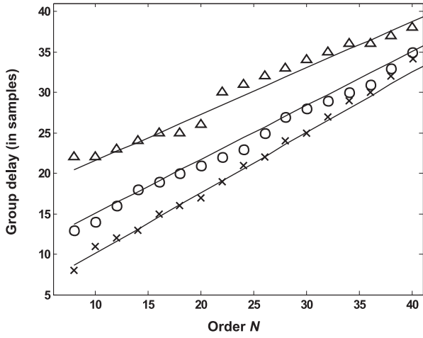
Fig. 3. The values of \tau_1 versus N for lowpass filters with M = 4 and \omega_t = 0.04\pi obtained for: \omega_{pw} = 0.05\pi ( \Delta ), \omega_{pw} = 0.1\pi (o), \omega_{pw} = 0.2\pi (x), and its approximation (solid lines) by (5).
