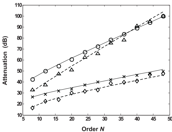
Fig. 4. Approximation of the stopband attenuation versus N for the lowpass filters with M = 6 and with: \omega_{pw} = 0.7\pi , \omega_t = 0.13\pi ( \Delta ), \omega_{pw} = 0.2\pi , \omega_t = 0.13\pi (o), \omega_{pw} = 0.2\pi , \omega_t = 0.04\pi (x), \omega_{pw} = 0.7\pi , \omega_t = 0.04\pi ( \diamond ).
