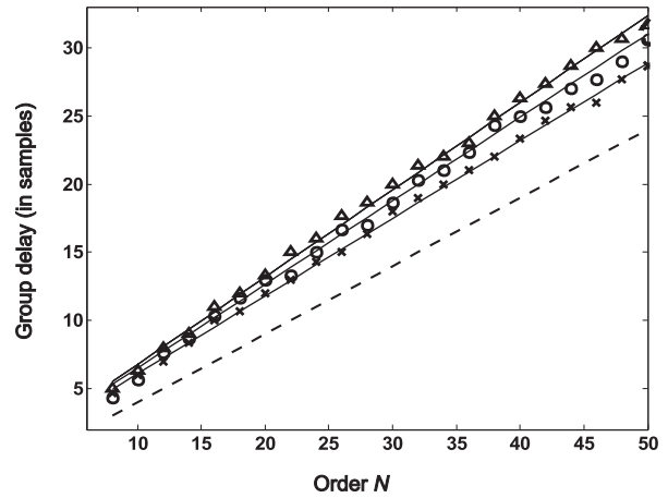
Fig. 1. The average values of \tau_1 versus N for lowpass filters with M = 2 obtained for: \omega_t = 0.04\pi ( \Delta ), \omega_t = 0.07\pi ( \circ ), \omega_t = 0.16\pi ( \times ), and its approximation (solid lines) by (5), \tau_{min} plotted for comparison (dashed line).
