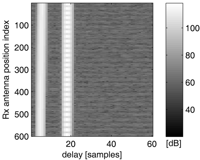
Fig. 5. The range profiles matrix of the simulated scene.
