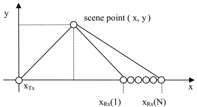
Fig. 7. The bistatic ground-based SAR geometry.
