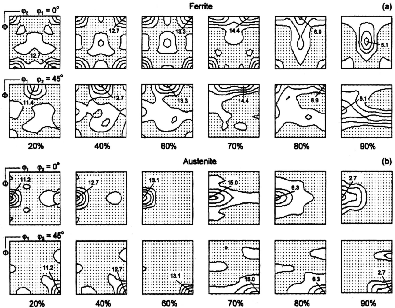
Fig. 2. Orientation distribution functions (ODFs) in sections \phi_1 = 0^\circ, \phi_2 = 45^\circ for ferrite (a) and in sections \phi_2 = 0^\circ, \phi_2 = 45^\circ for austenite (b) after the selected rolling reductions.
