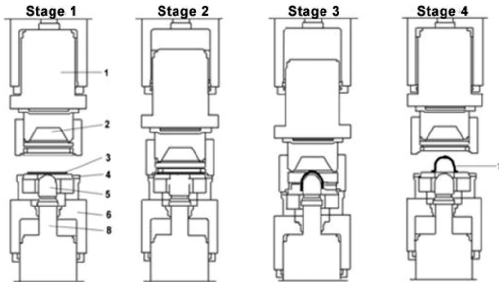
Fig. 13. Forming stages in the punch method: 1. main ram, 2. oil dome, 3. blank, 4. blank holder, 5. punch, 6. lower ram, 7. finished part, 8. column
