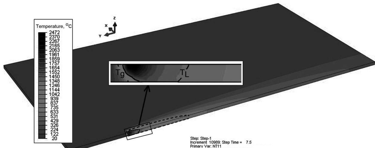
Fig. 4. Temperature profile in laser butt welded joint. Distribution at the top surface and in longitudinal section of the joint
