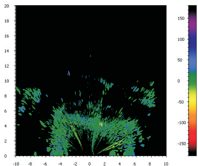
Fig. 8. Differential interferogram obtained on coherent images taken at different days.
