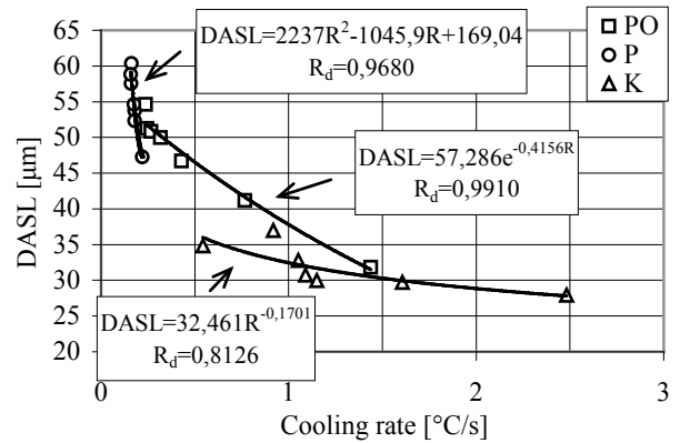
Fig. 7. Change of distance between arms in dendrites as a function of cooling rate
