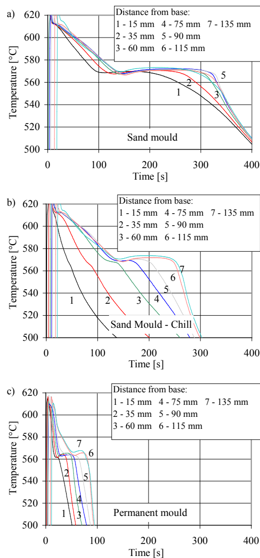
Fig. 4. Cooling curves of the plate casting, made in: a) sand mould, b) sand mould with chill, c) permanent mould
