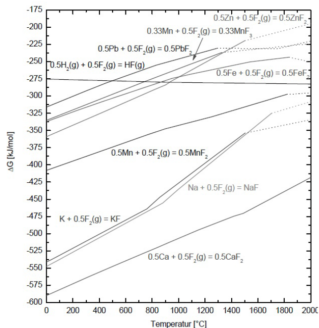
Fig. 2. The reactions of the enthalpy of single fluorides in the function of the temperature [3]
