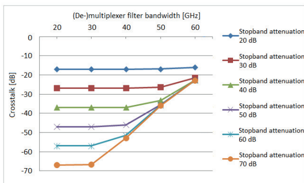
Fig. 12. Crosstalk values versus demultiplexer and multiplexer filter bandwidth for OOK modulation, 10 Gb/s bit rate and different stopband attenuation of rectangular filter characteristics.
