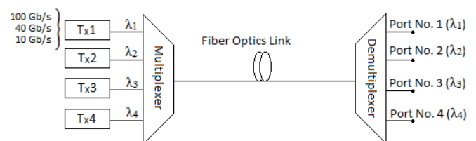
Fig. 1. Diagram of simulated DWDM system RX1, RX2 – receivers Schematics of simulated system; Tx1, Tx2, Tx3, Tx4 are transmitters of each wavelength: \lambda_1, \lambda_2, \lambda_3, \lambda_4 . Channel at the Port no.2 ( \lambda_2 ) was considered for calculating interchannel crosstalk.
