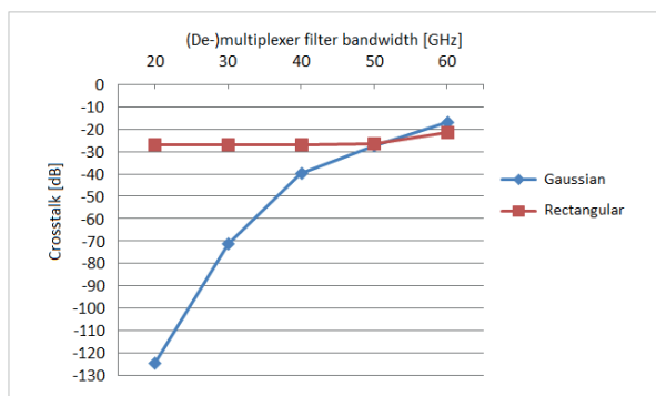
Fig. 13. Crosstalk values versus demultiplexer and multiplexer filter bandwidth for OOK modulation, 10 Gb/s bit rate and different types of filters: second order gaussian filter and rectangular filter with stopband attenuation 30 dB.
