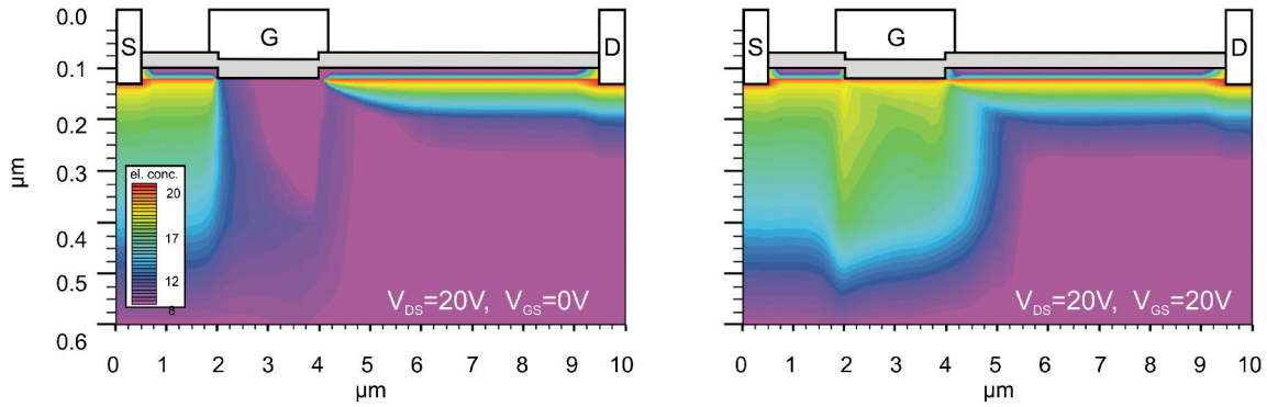
Fig. 3. The distribution of electron concentration in AlGaN/GaN MOS-HEMT in off- ( V_{DS}=20V, V_{GS}=0V ) and on-state ( V_{DS}=20V, V_{GS}=20V )
