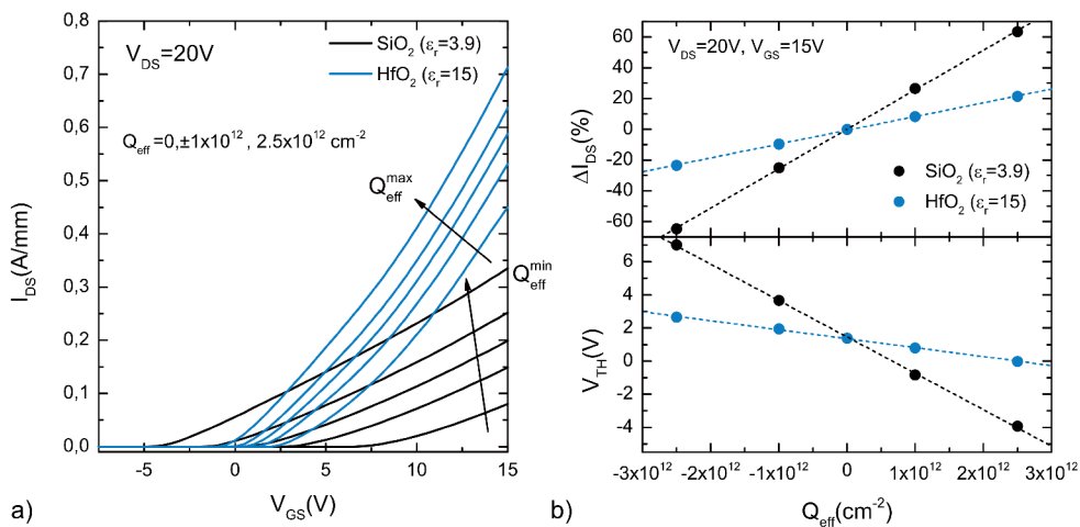
Fig. 8. The effect of effective charge density on a) AlGaN/GaN MOS-HEMT transfer characteristics and b) on-state current ( V_{DS}=20V , V_{GS}=15V ) and the threshold voltage for different gate dielectric SiO 2 ( \epsilon_r=3.9 ) and HfO 2 ( \epsilon_r=15 )
