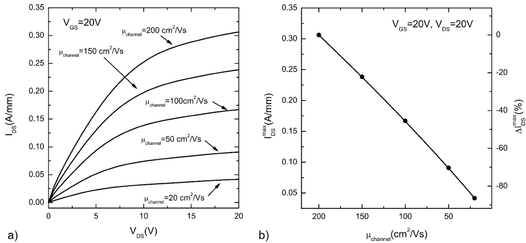
Fig. 7. The effect of channel mobility on a) AlGaN/GaN MOS-HEMT output characteristics and b) on-state current ( V_{DS}=20V , V_{GS}=20V )
