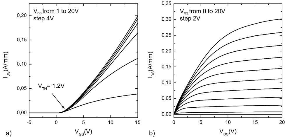
Fig. 4. Transfer (a) and output (b) characteristics of AlGaN/GaN MOS-HEMT
