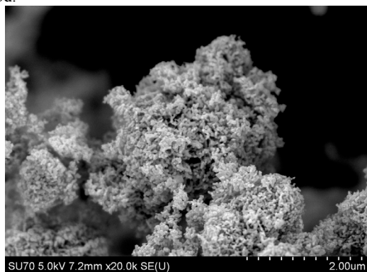
Fig. 2. SEM image of ZnO nanoparticles, magnification: 20 [4]
