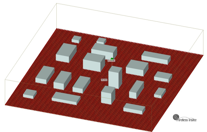
Fig. 5. Remcom Wireless InSite - Project View: scenario 5 and 6. Transmitter (green point) between eighteen concrete buildings (gray). Square terrain covered by grid of receivers (red points).
