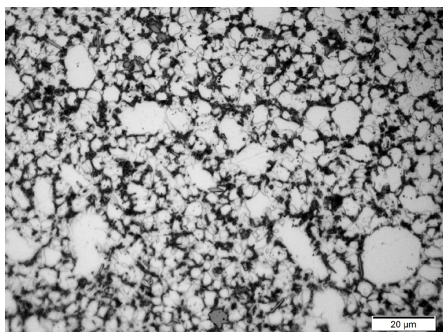
Fig. 4. Microstructure of high-pressure die-casting AME505 magnesium alloy
