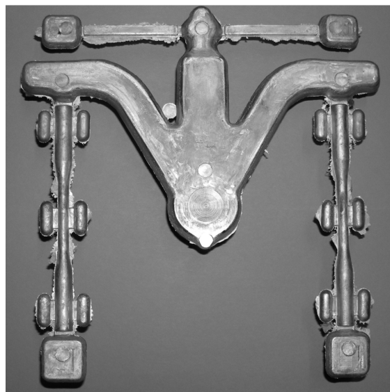
Fig. 1. Macrograph of AME505 experimental magnesium alloy cast fabricated by IDRA-380 cold-chamber die-casting
