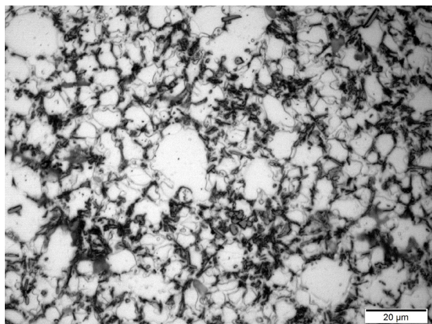
Fig. 3. Microstructure of high-pressure die-casting AME503 magnesium alloy
