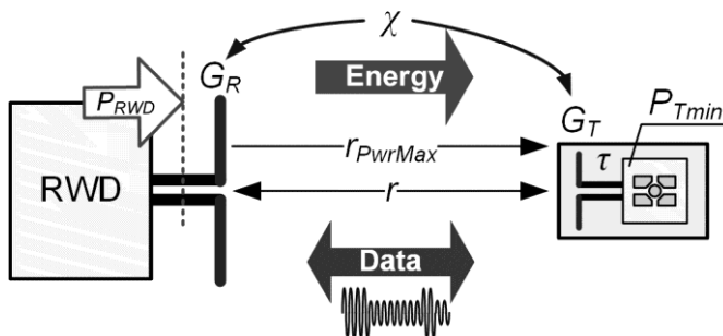
Fig. 2. Communication system of RWD - transponder arrangement in UHF band.
