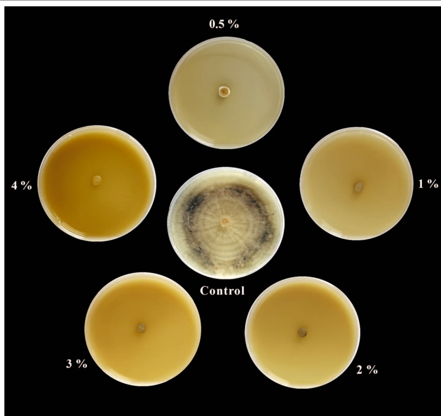
Fig. 1. Effect of different concentrations of clove extract on the radial growth of R. solani
