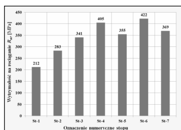
Fig. 2. Graphical presentation of the results of numerical calculations (for the measuring point Pkt 1): a) the tensile strength R_m and b) the elongation A (see Table 5)
