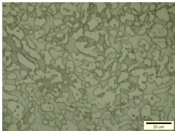
Fig. 5. Metallographic image of the etched duplex steel structure
