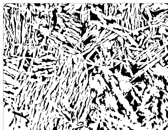
Fig. 4. Metallographic image of the etched cast iron matrix structure after graphical processing by INSCAPE
